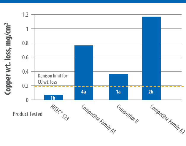
HiTEC® 523 Based Oil Versus Several Commercially Available Competitor Products in the ASTM D2619 Hydrolytic Stability Test
